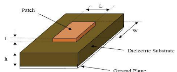
Fig.1: Structure of Rectangular Microstrip Patch Antenna
