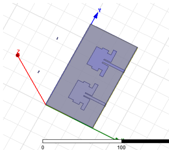
Fig.2 Geometry of 2 port MIMO Rectangular Patch Antenna
