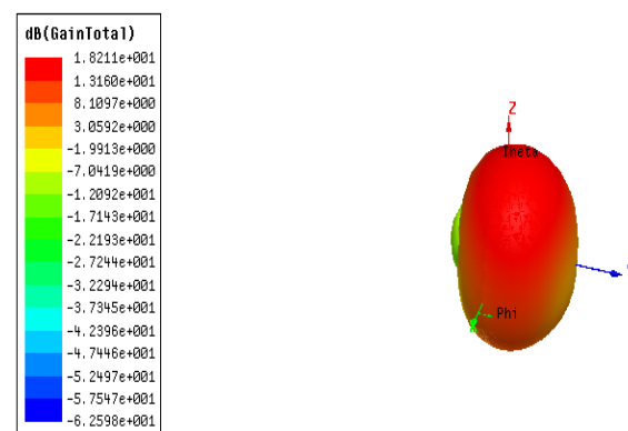
Fig.4. Total Gain of 2 port MIMO antenna
