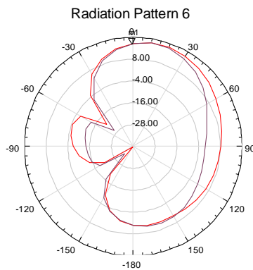
Fig.5. 2D radiation pattern of 2 port MIMO antenna
