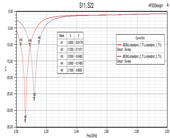
Fig.3. Return Loss (S11, S22) of 2 port MIMO antenna using FR4 material
