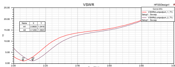
Fig.6. Graph of VSWR vs Frequency
