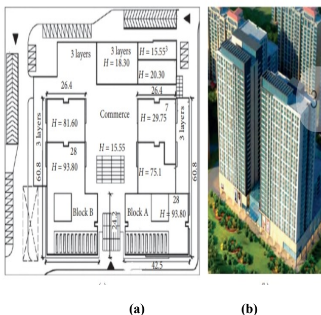
Figure 1: General plan and the architectural effect drawing of an enlarged base multitower high-rise building (a) General plan of building/m (b) Architectural renderings.
