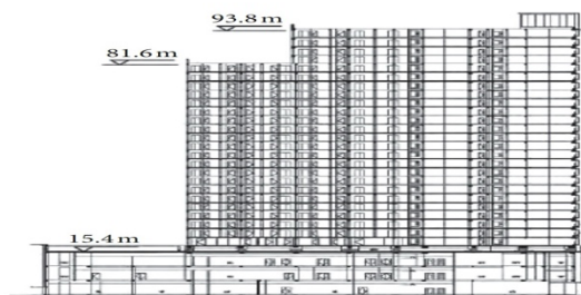
Figure 2: Schematic architectural section of tower B.
