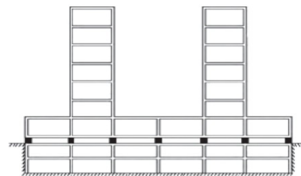
Figure 4: Base isolation diagram of the first floor.
