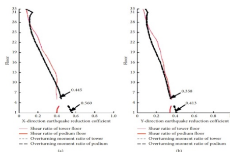
Figure 14: Horizontal earthquake reduction coefficient of tower
