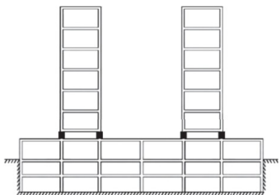
Figure 5: Schematic diagram of interlayer isolation.
