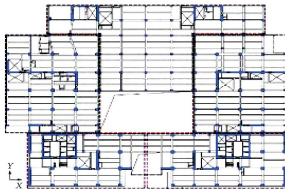
Figure 3: Joint drawing of the traditional seismic scheme.
