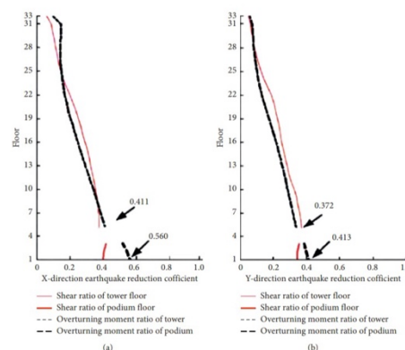
Figure 13: Horizontal earthquake reduction coefficient of tower A
