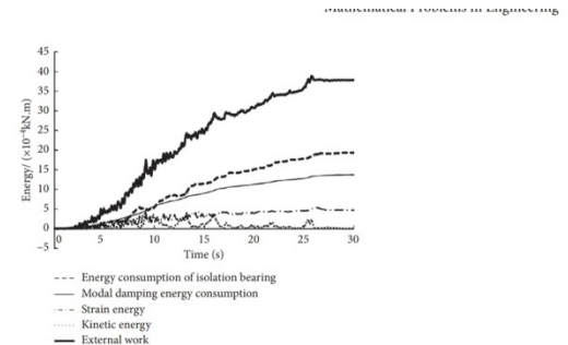
Figure 17: Energy curve of structure under artificial wave Y main direction earthquake action
